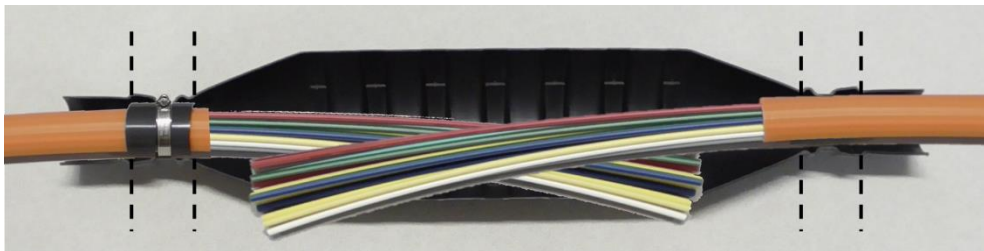
1.10 Following insert second duct bundle into bottom shell at opposite side. Fixation just takes place after connection of microducts.
