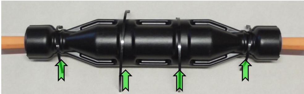
1.17 Position top shell onto bottom shell in a manner, bottom shell slides into groove at top shell.
