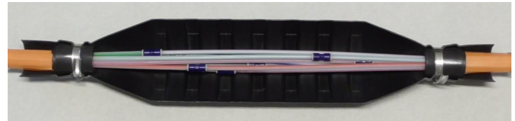
1.15 After all microducts have been connected, still loose side of microduct bundle need to be fixed. Install rubber stripe and duct bundle strain release as described under chapter 1.6 and following. Before fixing of hose clamp, check again if rubber stripe and clamp shell are in right position. Right position is mandatory for full strength of strain relief. Afterwards tighten hose clamp like described under chapter 1.9.
