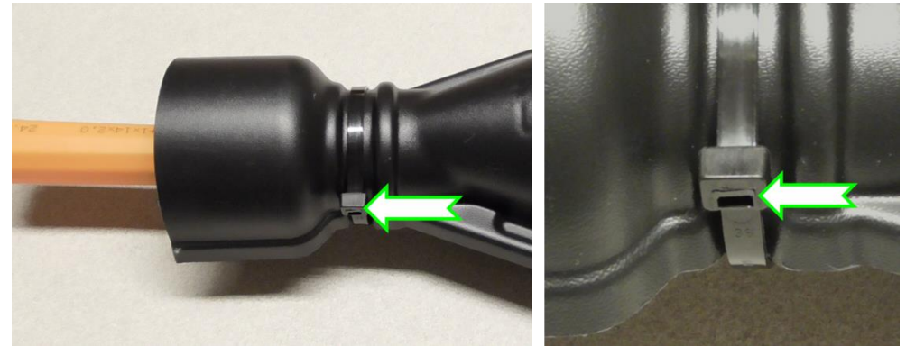
1.19 Cut cable ties flush with a side cutter. (No risk of injury caused by sharp edges)
