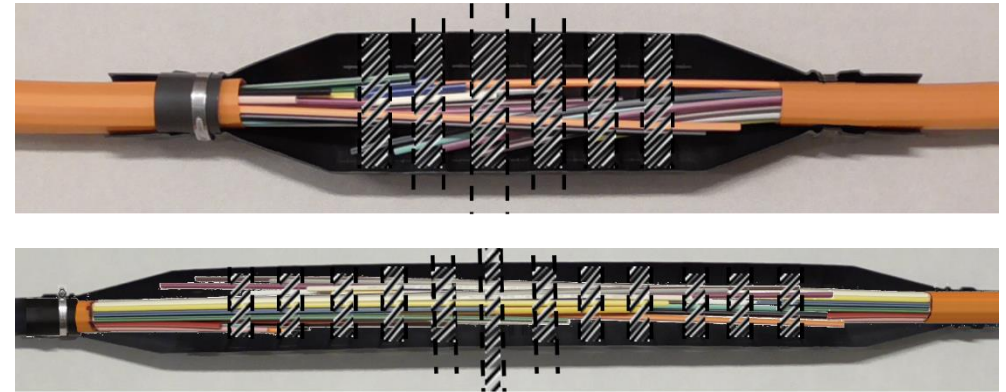
1.12 The connectors for joint of microducts have to be distribute graded over the inner space of DuctShell. This ensure max capacity and prevent cable stops during jet in. In order to do so, connect microducts according to customers colure code.
